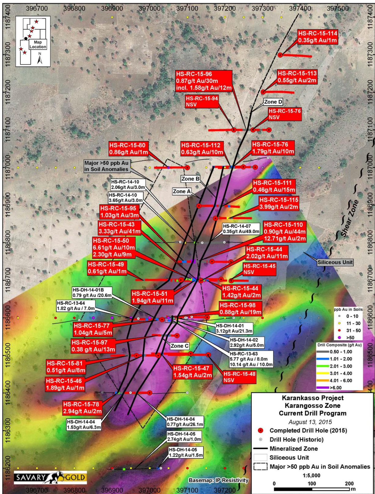
Figure 1. - Karangosso Zone – Surface Plan and Assay Summary
